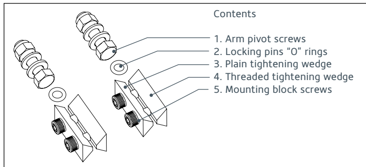
BM ARK - For Mounting Blocks & V-Trak arms
