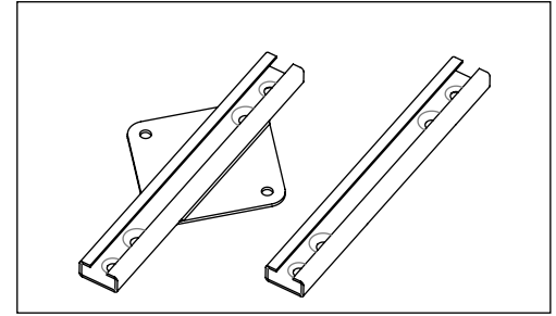
TP / T - Tracks
